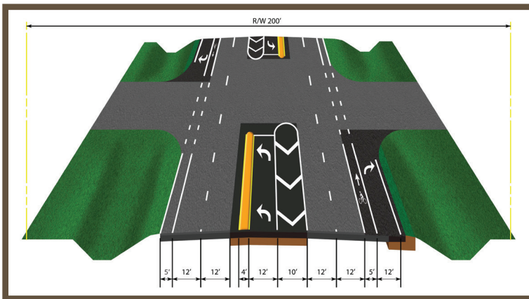
Proposed features on U.S. 90A (East Nine Mile Road) from County Road 749 (Chemstrand Road) to Baldrige Drive:
