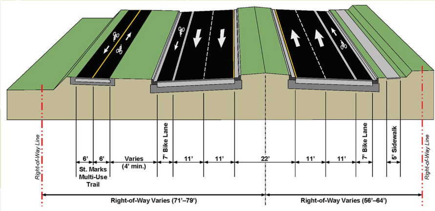
S.R. 363 (Woodville Highway) Four-Lane Urban Typical Section
