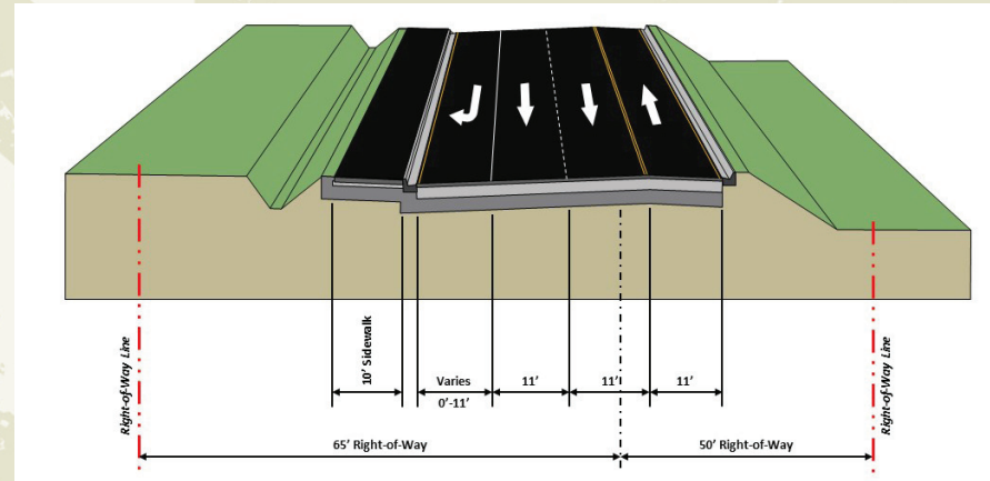
Tram Road Three-Lane Urban Typical Section with Turn Lane
