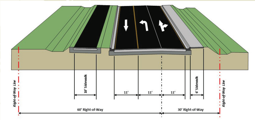
Ross Road Two-Lane Urban Typical Section with Turn Lane
