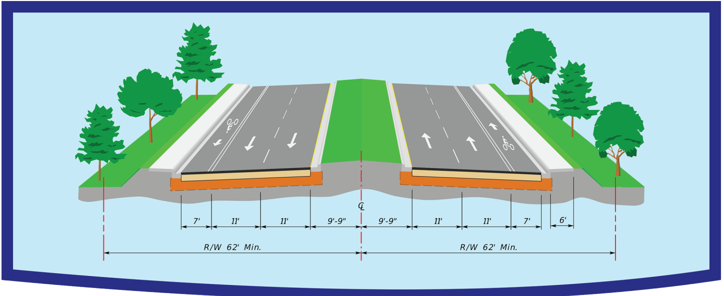
Four-Lane Urban Typical Section
